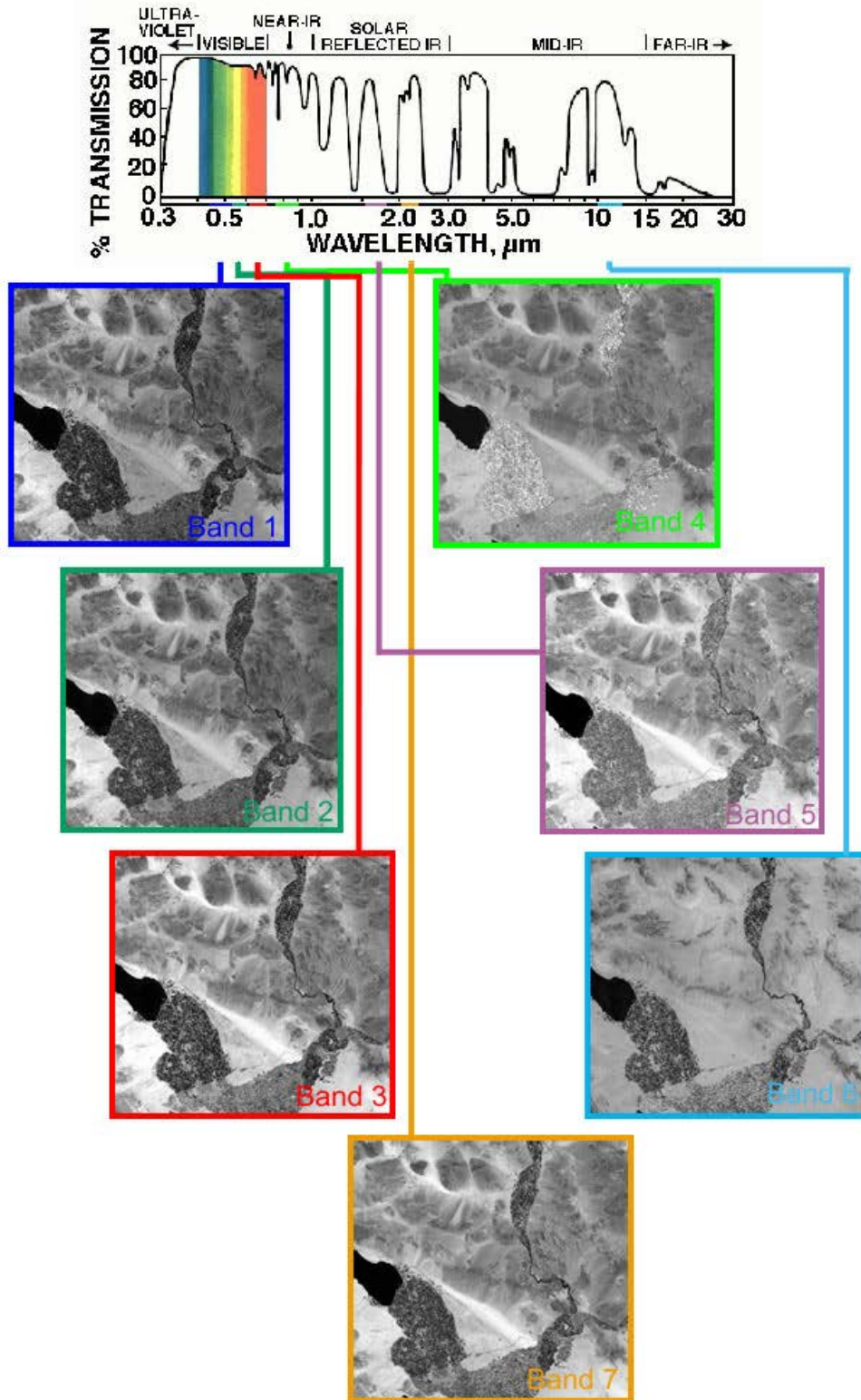
Electromagnetic Spectrum Image from Virtual Hawaii .
